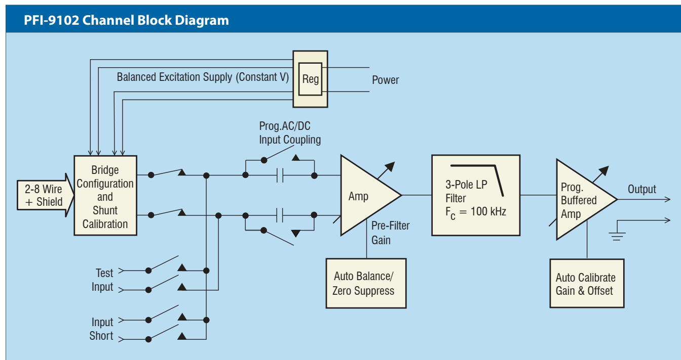
PFI-9102 Channel Block Diagram
