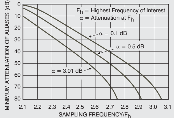
LP8F ATTENUATION OF ALIASES VS SAMPLING FREQUENCY
