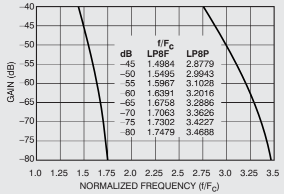
LP8F & LP8P TRANSITION REGION AMPLITUDE RESPONSE
