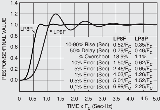
LP8F & LP8P STEP RESPONSE
