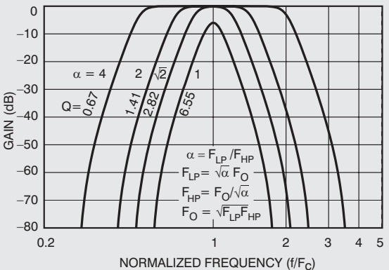
BANDPASS AMPLITUDE RESPONSE HP8F & LP8F CASCADED
