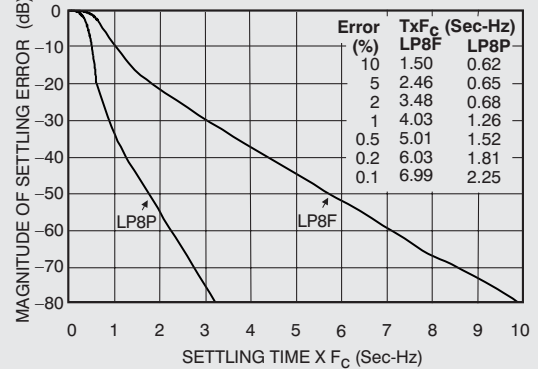
LP8F & LP8P SETTLING TIME
