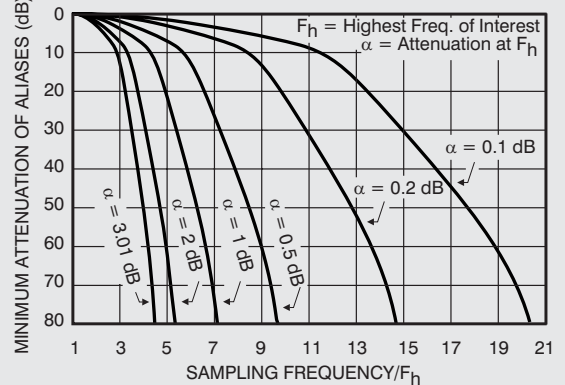
LP8P ATTENUATION OF ALIASES VS SAMPLING RATE
