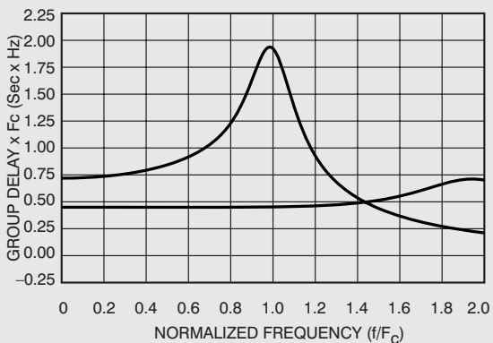
LP8F & LP8P GROUP DELAY
