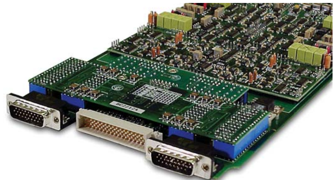
The 28104A Card with Bridge Configuration Module.
