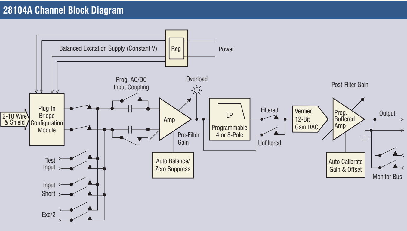
28104A Channel Block Diagram
